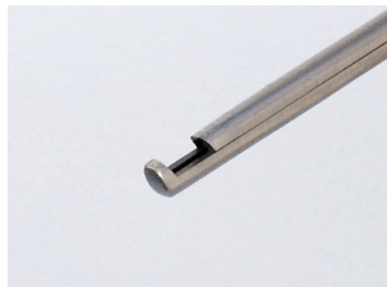
Ferris-Smith Punch, 180x3mm, 40° up-angled
